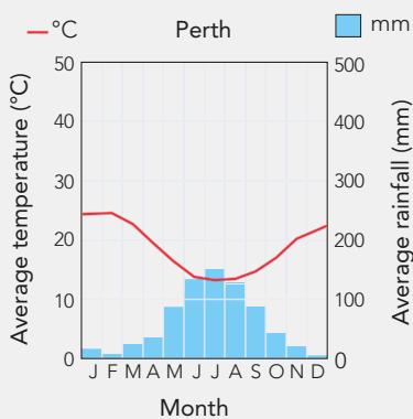
Source 29 A climate graph showing the average monthly temperature and rainfall in Perth
