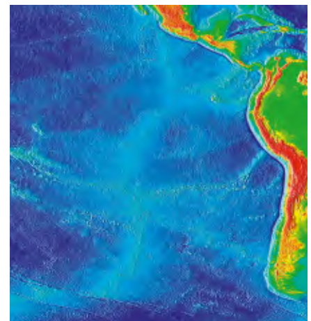
Figure 5.15 A topographical image of the East Pacific Rise off the west coast of South America. The red, yellow and green indicate higher points.
