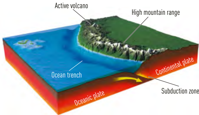
Figure 5.19 Ocean-to-continent collision causes subduction. It creates mountains, volcanoes and an ocean trench.
