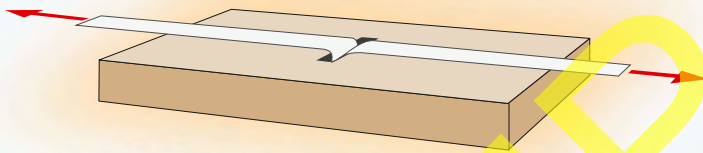
Figure 5.31 Slowly pull the strips of paper away from each other.
