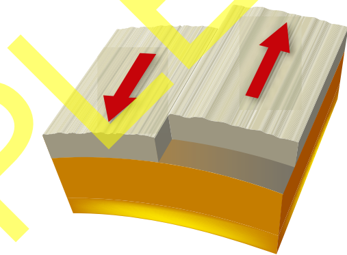
Figure 5.16 Transform boundaries: one plate slides against another.
