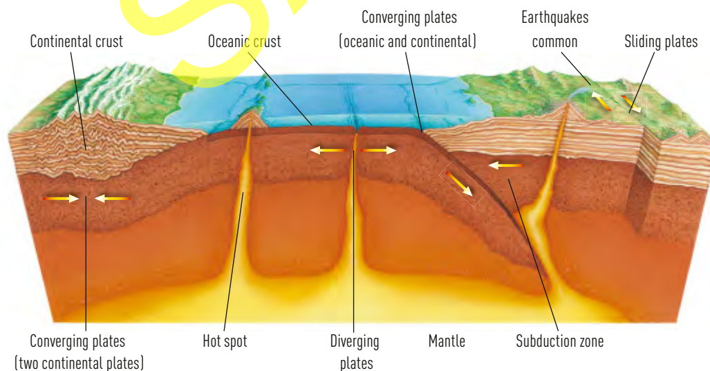
Figure 5.8 Some common landforms created as a result of tectonic plate movement.
