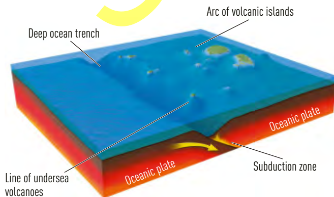
Figure 5.21 Ocean-to-ocean collision causes subduction. It creates a trench and a line of undersea volcanoes.
