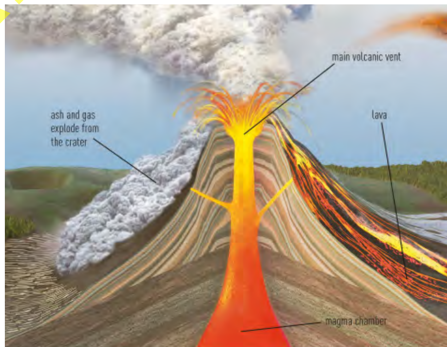
Figure 5.10 Cross-section of an active volcano.
