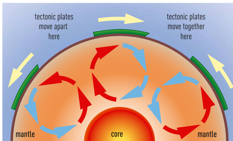
Figure 5.3 Continental drift is explained by the convection currents of the mantle below the solid crust of the tectonic plates.
