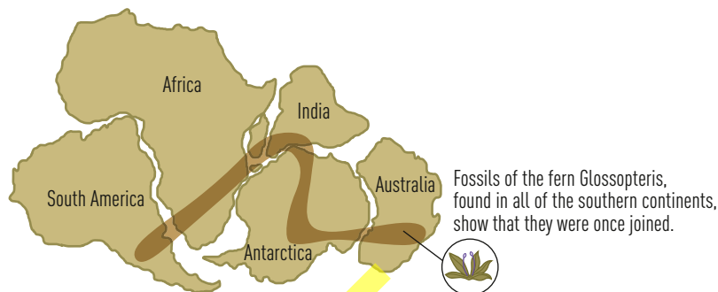
Figure 5.2 Given that the fossil fern Glossopteris cannot walk, swim or fly, how can its isolated occurrence in so many different parts of the world be explained?
