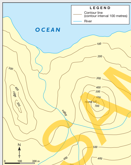
TOPOGRAPHIC MAP SHOWING A ROUND HILL, A VALLEY AND A RIDGE
