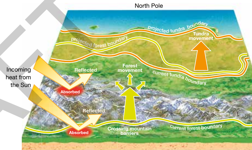
Source 2 The movement of tundra (frozen, treeless land) and forests towards the North Pole in the Arctic. As mountain slopes become forested they absorb more heat from the Sun rather than reflecting it, further increasing temperatures.
