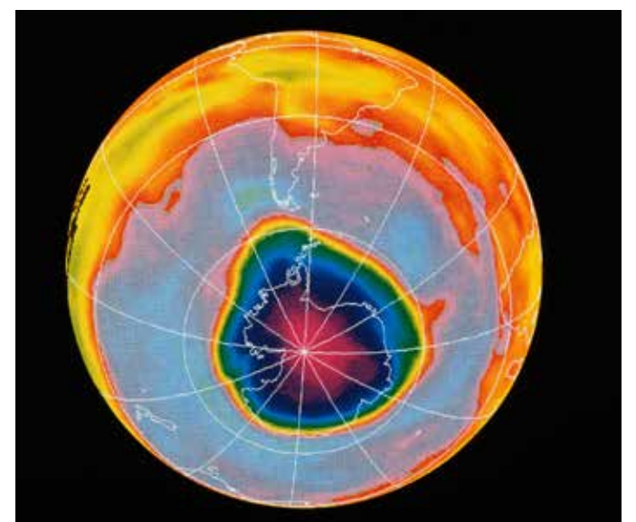
Source 3 A satellite map showing a severe depletion or 'hole' in the ozone layer over Antarctica on 3 October 1990. The hole appears here as the violet and pink areas covering Antarctica (outlined in white) and beyond.
