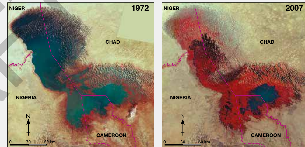
Source 3 Satellite images of Lake Chad in 1972 and 2007
