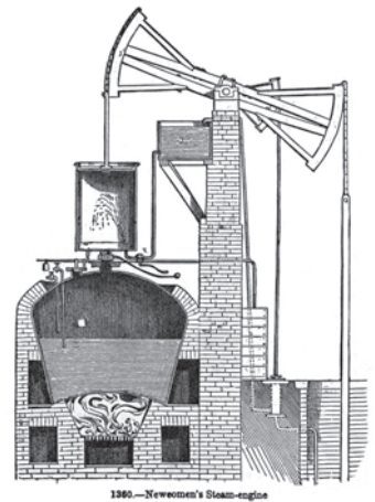
1360.—Newcomen's Steam-engine
